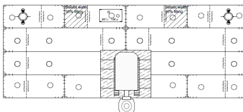
Drilling configuration
