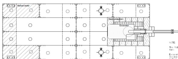
Excavator configuration
